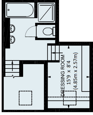
MEZZANINE
