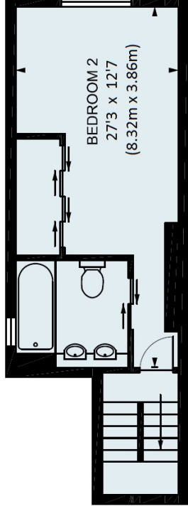
SECOND FLOOR
