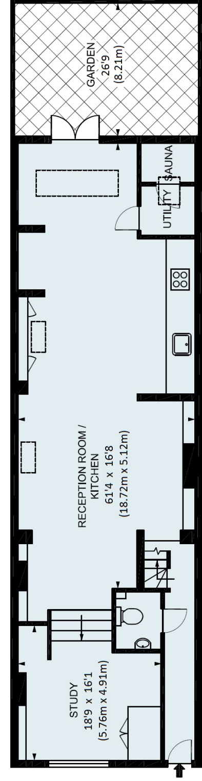
GROUND FLOOR
